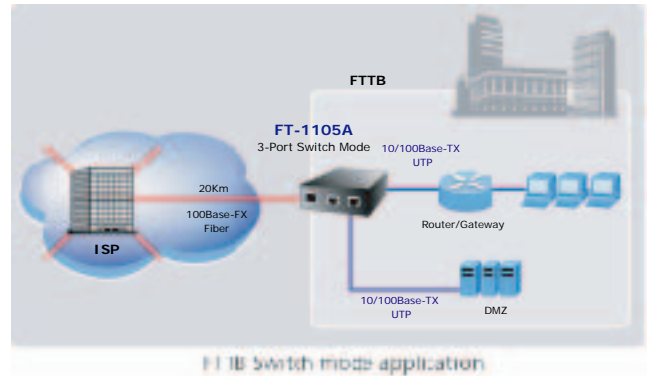
Intranet Link path redundant Fiber to two Copper switch mode for FTTx applications
