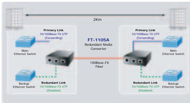
Intranet Link path redundant Fiber to two Copper switch mode for FTTx applications
